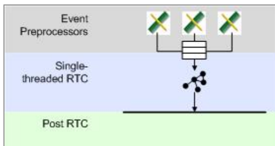
Figure 10: Single-Threaded RTC
