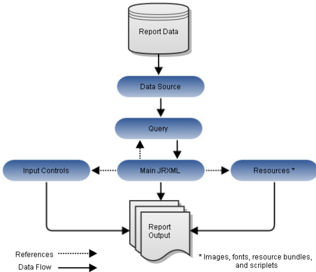
Figure 7-1 Anatomy of a Report Unit
