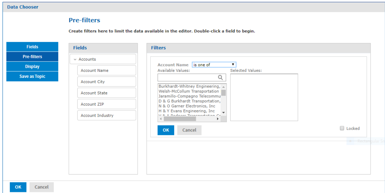
Figure 5-25 Condition Editor in the Filters Panel on the Pre-filters Page
