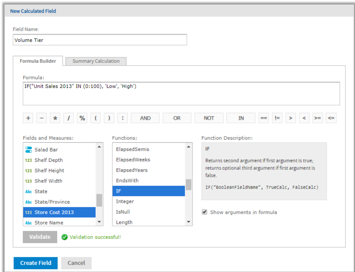
Figure 5-19 Formula Builder Tab in New Calculated Measure Dialog Box
