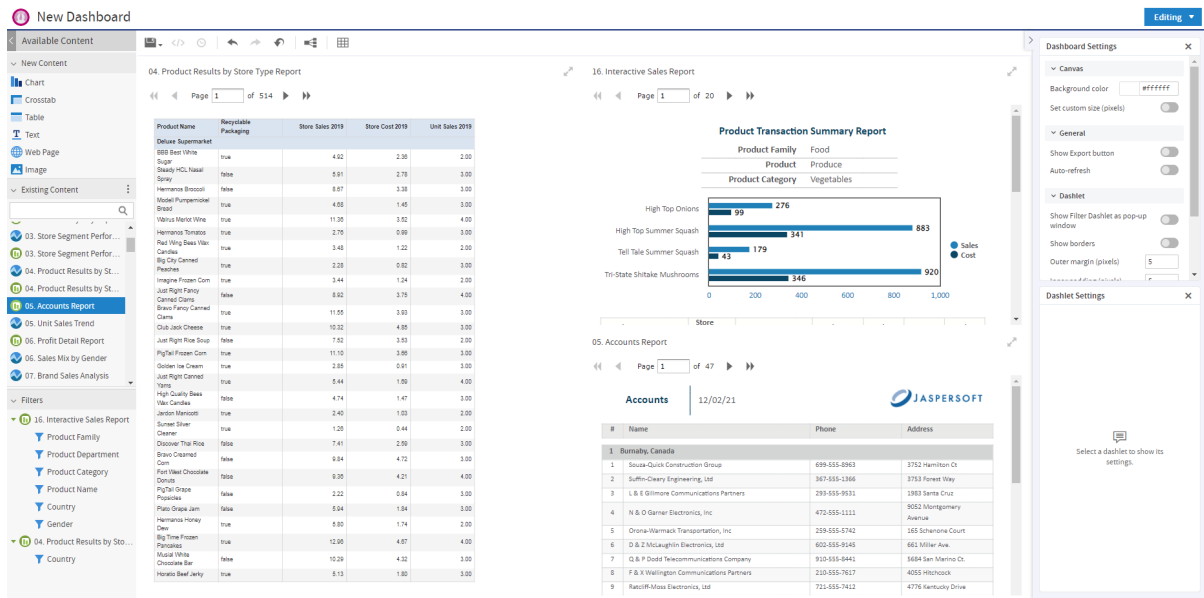
Figure 2-14 Simple Dashboard Canvas with three reports
