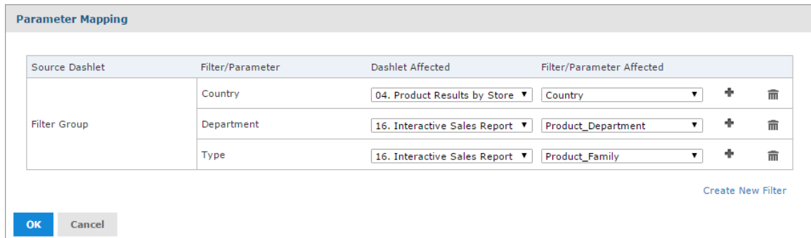
Figure 2-12 Parameter Mapping for the Sales Dashboard
