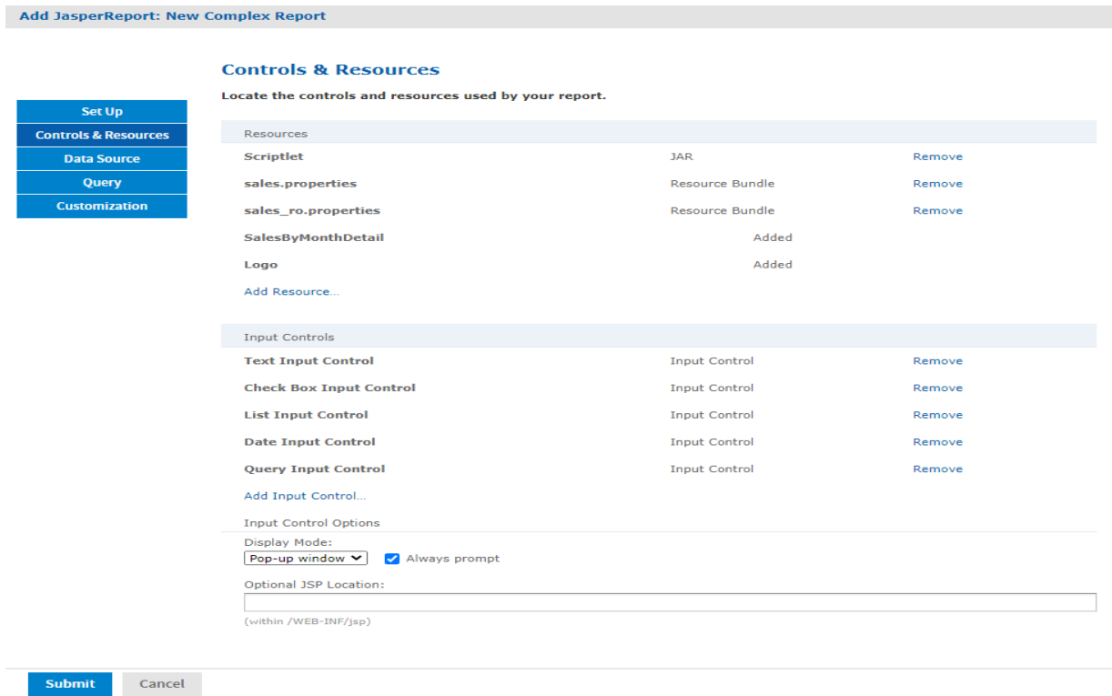
Figure 7-22 Input Controls and Resources
