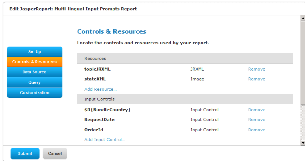
Figure 5-42 Input Controls Include One Multi-lingual Input Control
