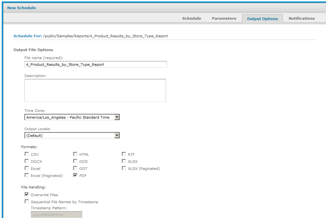
Figure 3-16 Output Page for Scheduling a Report – Output File Options
