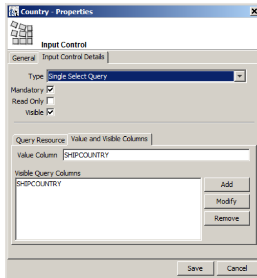
Figure 7-8 Properties of an Input Control Resource
