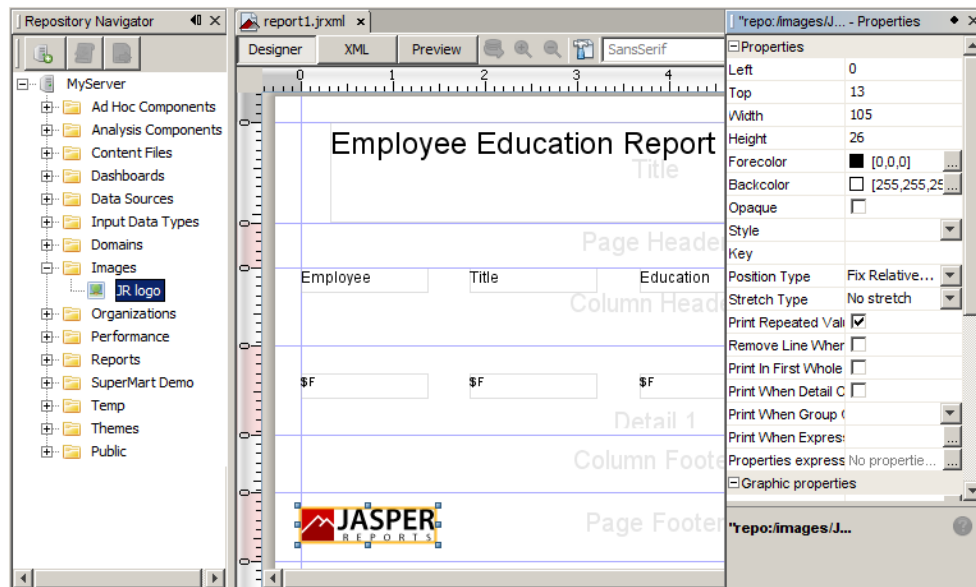
Figure 7-5 A Repository Image Added to a Report
