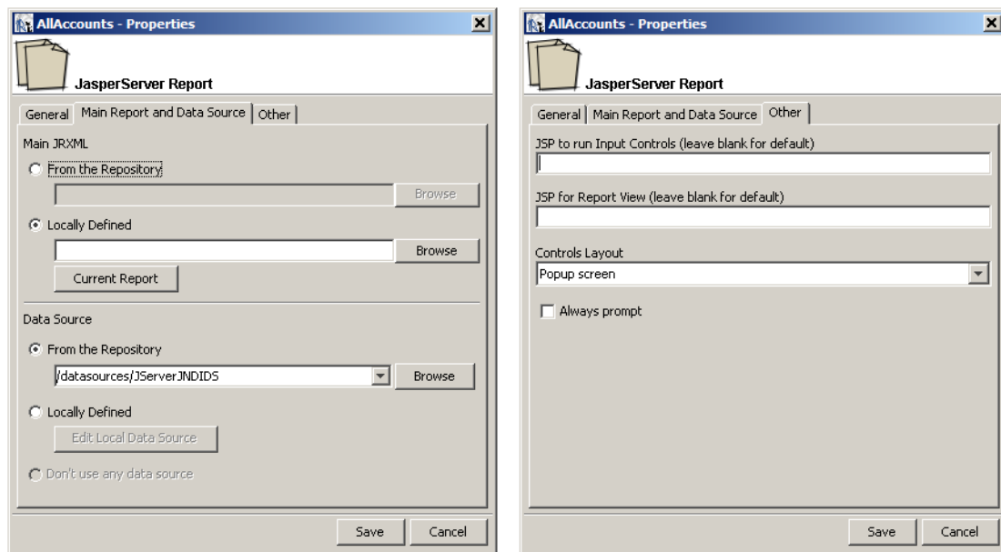
Figure 7-9 Properties of a Report Unit in iReport
