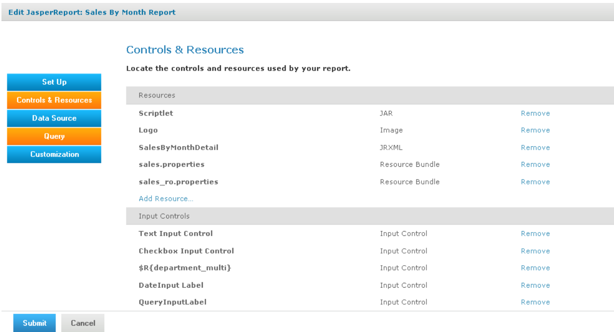
Figure 5-34 Controls & Resources Listing Only One Input Control
