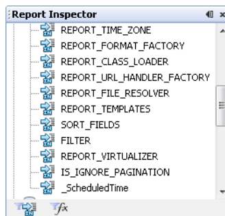
Figure 3-22 _ScheduledTime Parameter in the Report Inspector
