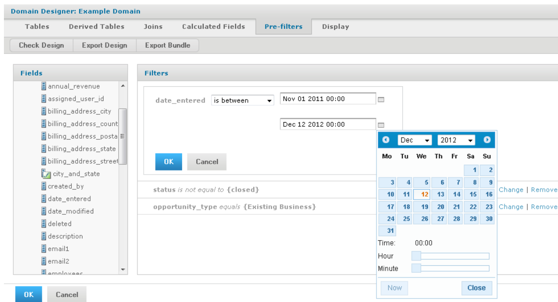
Figure 6-23 Filters Panel of the Domain Designer
