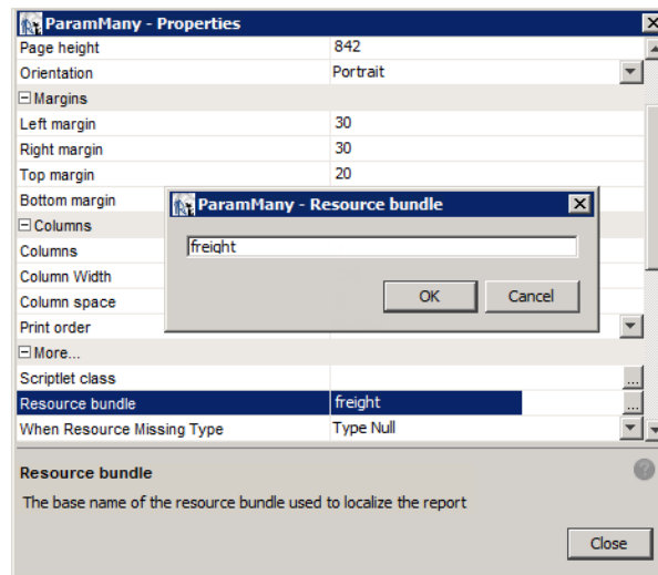
Figure 5-38 Setting the Base Name of the Resource Bundle
