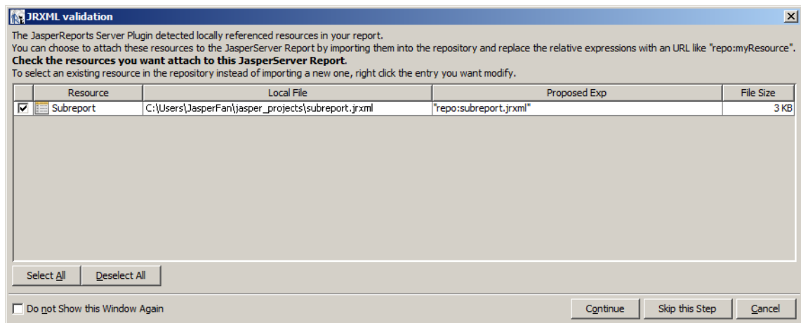
Figure 7-7 JRXML Validation
