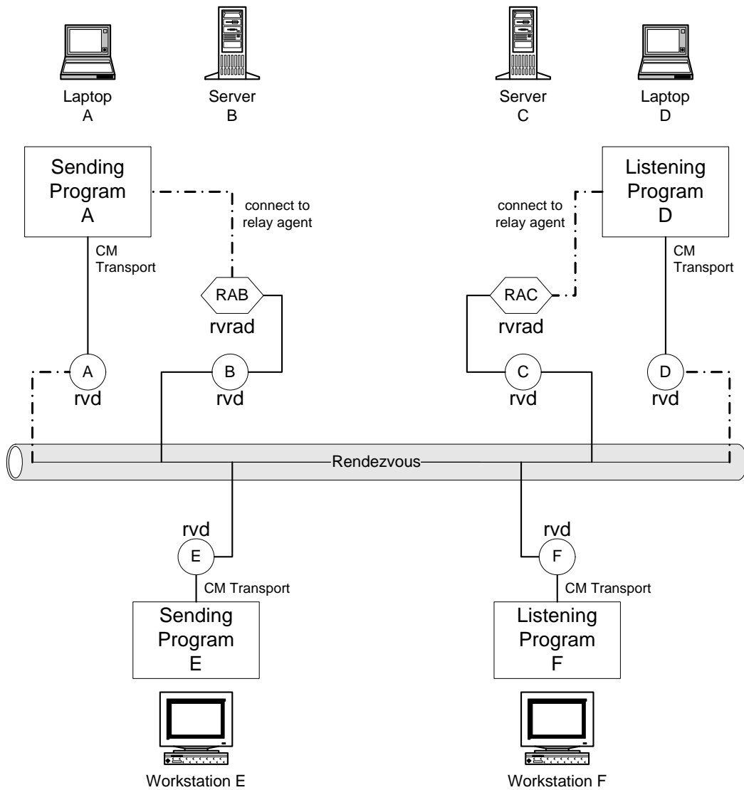
Figure 14 Relay Agents
